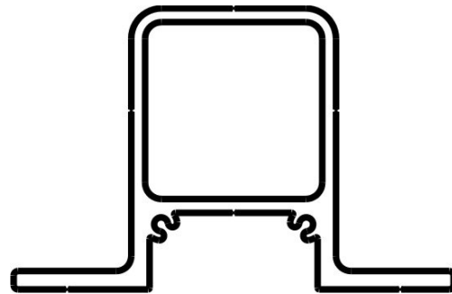
1" Intermediate Fascia Mount Bracket (6")
