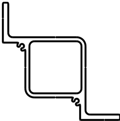
Inside Corner Bracket (6")
