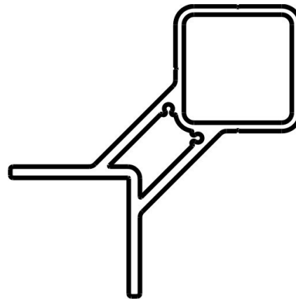
Outside Corner Bracket (6")
