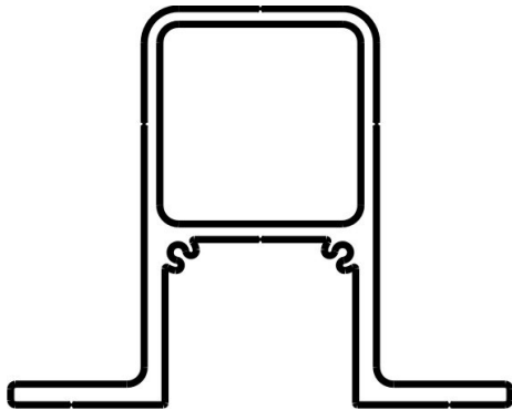
2" Intermediate Fascia Mount Bracket (6")
