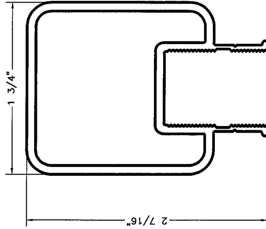
SERIES 375 TOP RAIL
