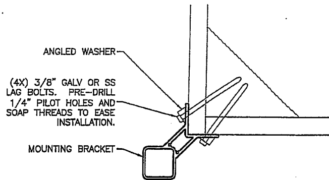
⑤ TYP CORNER FACE MOUNT PLAN VIEW 1\ 1/2"=1'-0"
