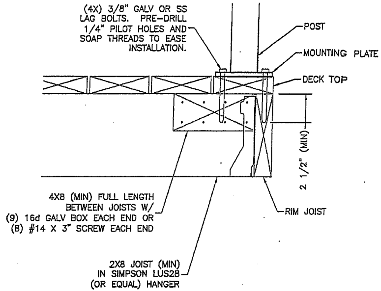
③ TOP MOUNT PERPENDICULAR TO JOISTS 1\ 1/2"=1'-0"
