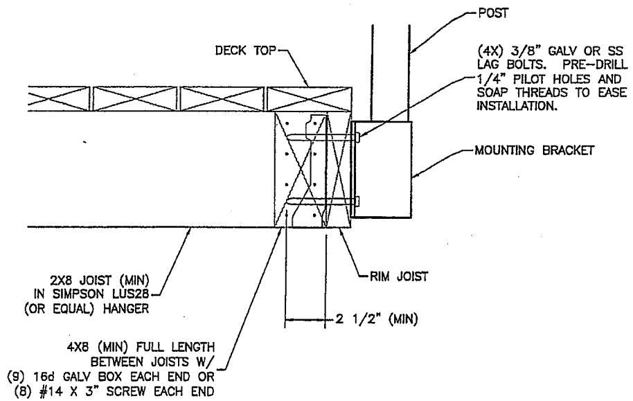
④ FACE MOUNT PERPENDICULAR TO JOISTS 1\ 1/2"=1'-0"
