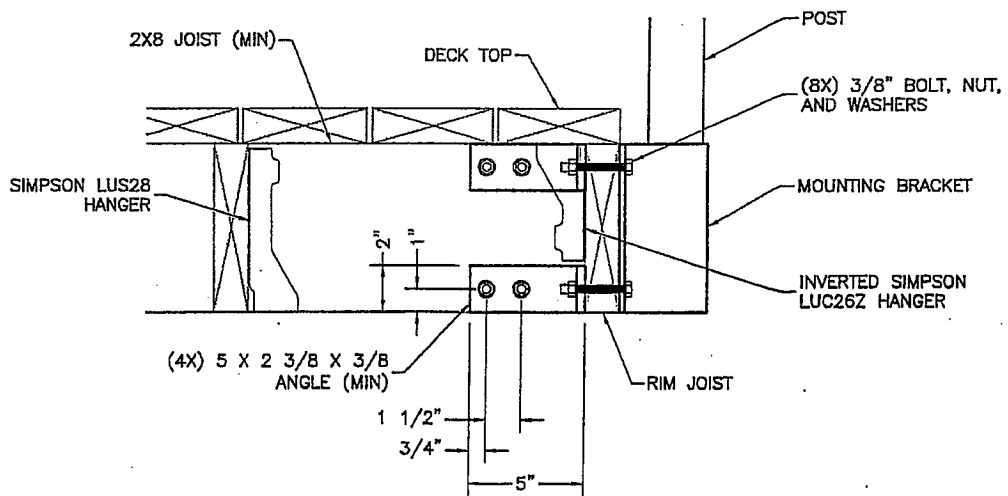
② FACE MOUNT PARALLEL TO JOISTS 1 1/2"=1'-0"
